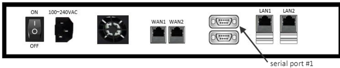
Figure 8. The ESBC 10K back panel
