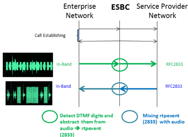
Figure 100 DTMF transcoding: G.711 in-band and RFC2833 processes
