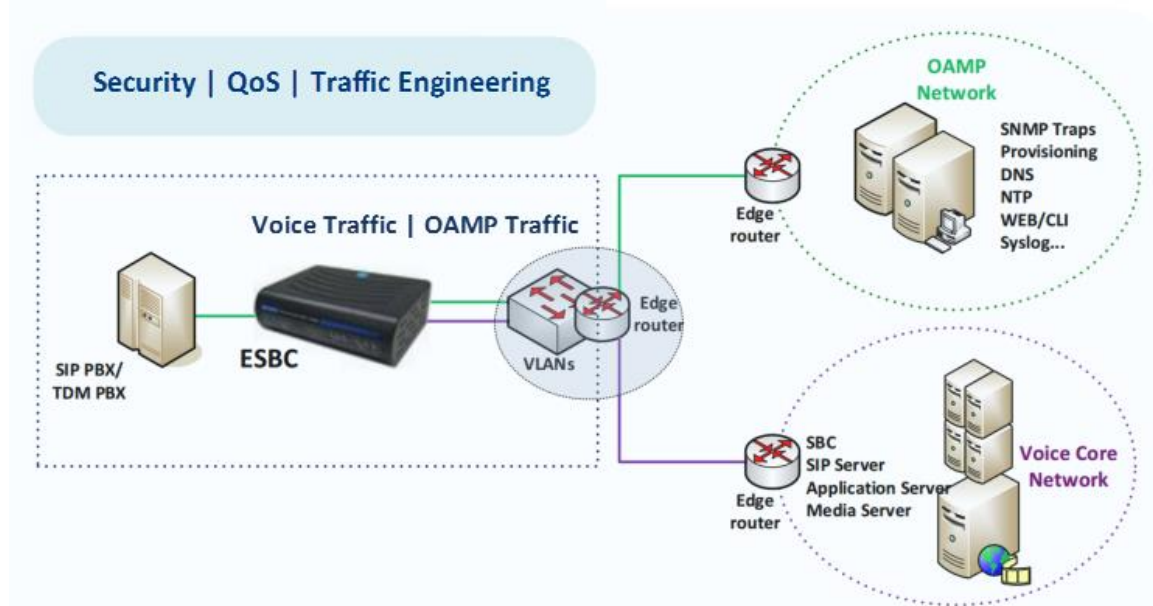
Figure 26. Multiple subnet architecture example for SIP Trunk voice service
