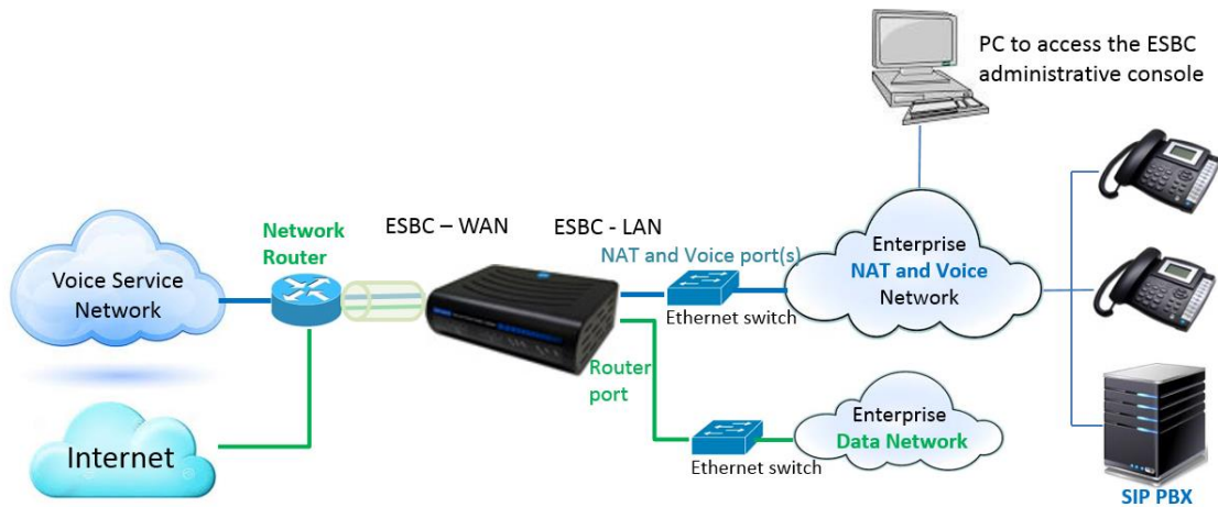
Figure 45. Enabling the ESBC Router Port for Data Service
