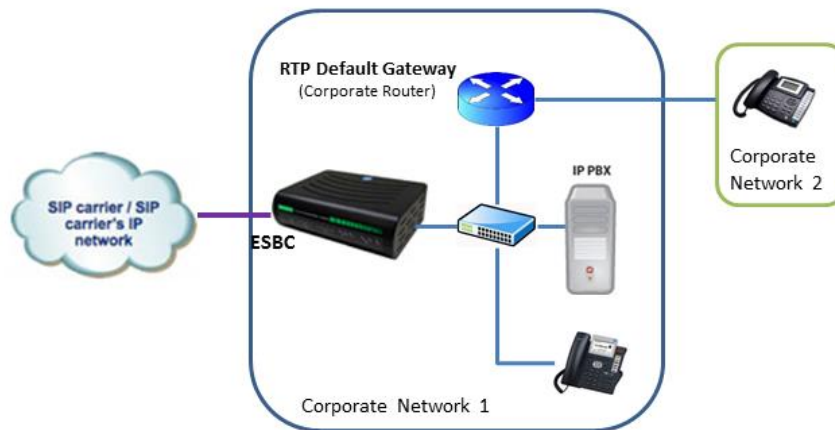
Figure 35. The enterprise Router acting as the RTP default gateway for SIP devices
