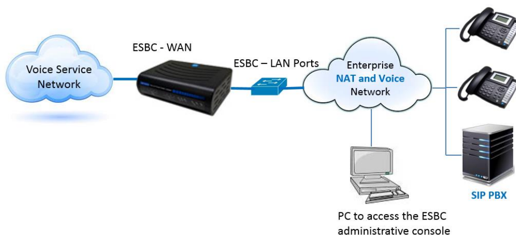
Figure 33. Default configuration: LAN ports serve enterprise telephony services
