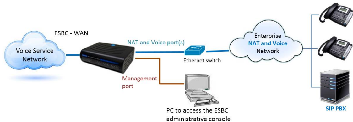
Figure 42. Enabling the ESBC management port
