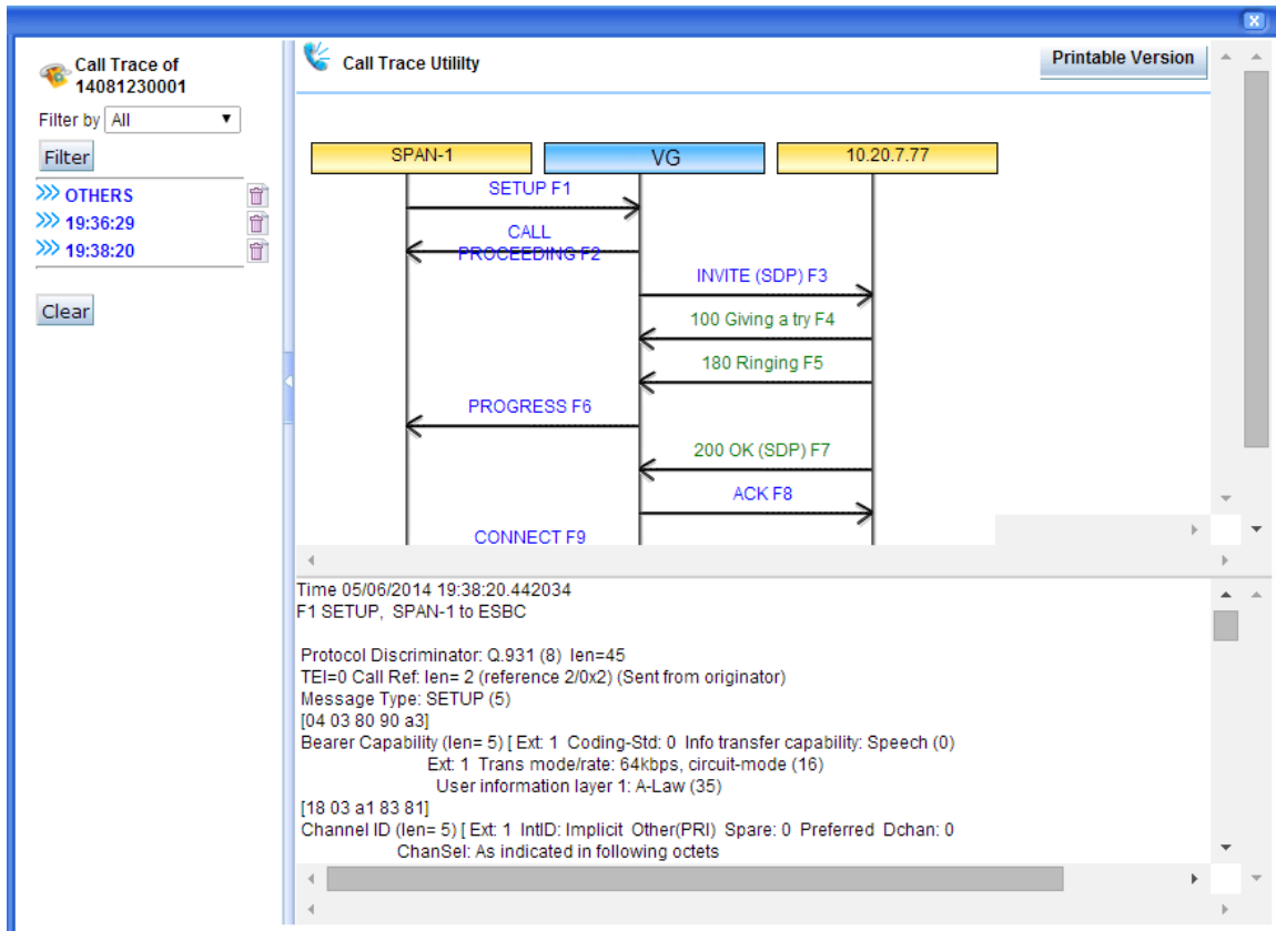
Figure 144. SIP and PRI signal trace of the selected account and call
