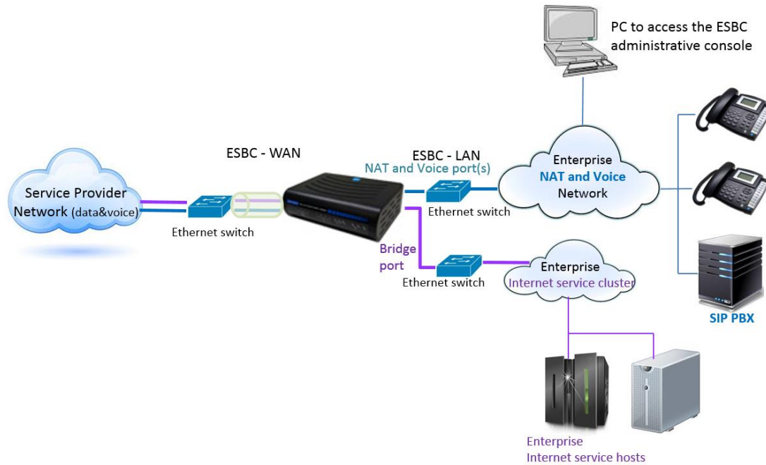
Figure 44. Enabling the ESBC Bridge Port for Enterprise Internet Service Hosts
