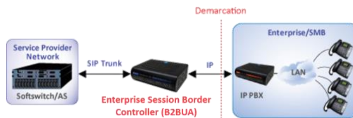
Figure 2. SIP Trunking Using ESBCs with B2BUA
